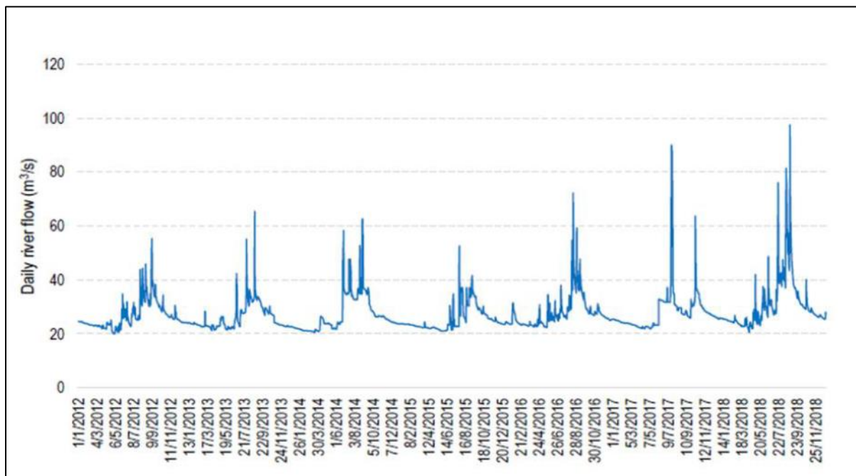
Figure 3: Example of river discharge (hydrograph) data, Nam Xam river, Sam Neua. Details of monitoring station not known. (Source: Earth Systems, 2021).
