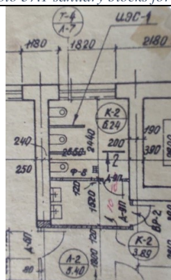
Figure 37.3 right wing sanitary block
