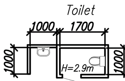
Figure 37.4 WASH facilities kitchen staff
