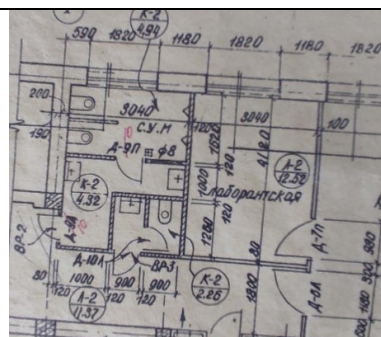
Photo 37.2 left wing sanitary block 2 nd floor
