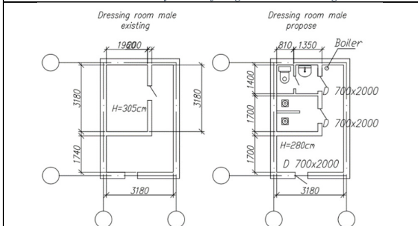
Photo 12.7 Shower and sanitary block sports hall locker room for boys
