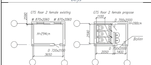
Photo 12.9 Wash facilities 2 nd floor, girls
